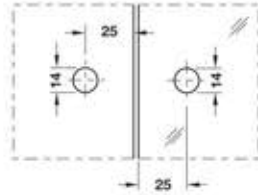
Size & Cutout Details for TCH-8439, TCH-8439 A & TCH-8439 R Glass to Glass 135° Connector
