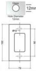
TCH-8507 Sliding Handle (Rectangle)
