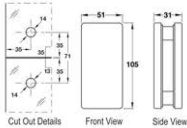
TCH-8416 Glass to Glass Connecting Patch with Wall/ Ceiling
