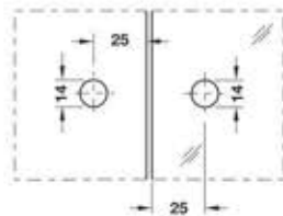
Size & Cutout Details for TCH-8443, TCH-8443 A & TCH-8443 R Glass to Glass 180° Connector
