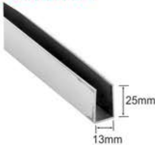
TCH-8467 (CP) U Channel (For Fixed Glass) Available in 3 Mtr. Thickness: 1.5mm Material : SS 304
