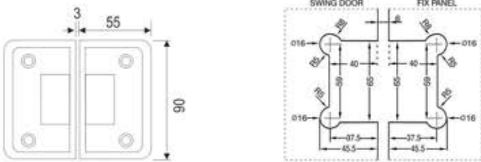
Size & Cutout Details for TCH-8427 & TCH-8433 Glass to Glass 180° Hinge
