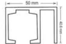
TCH-8514 One Fix and One Movable Glass Specification • Size : 8 Ft., 10 Ft., 12 Ft.
