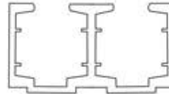
TCH-8513 Aluminium Sliding Double Track Specification • Size : 8 Ft., 10 Ft., 12 Ft.
