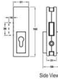
TCH-8407 Corner Patch Lock with Strike Plate
