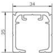
TCH-8828 Sliding Top Track
