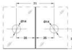
Cut Out Details
