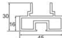
TCH-8829 Top/ Bottom Profile
