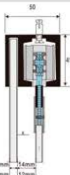
TCH-8514 Aluminium Track (Door+Fix Glass) Available in 8, 10 & 13 Ft.
