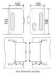
TCH-8506 Sliding Handle (Square)
