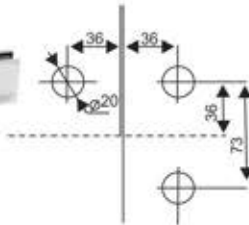
Cut Out Details
