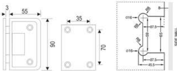
Size & Cutout Details for TCH-8425 & TCH-8431 Wall to Glass 90° Off Set Hinge
