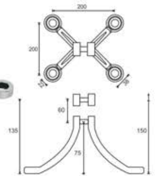
TCH-8838 Four Way Spider (Wall Mounted)
