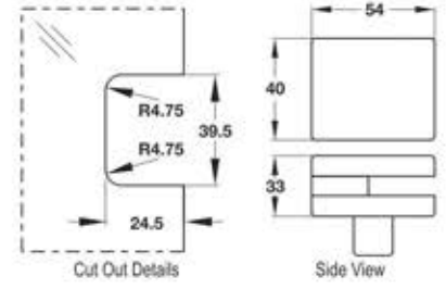
TCH-8411 Center Lock Strike Box
