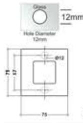
TCH-8507 Sliding Handle (Rectangle)
