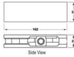
TCH-001 BM Top Patch
