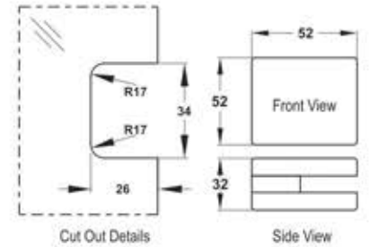
TCH-8415 Wall to Glass Connecting Patch
