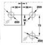
Cut Out Details
