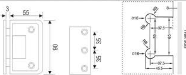
Size & Cutout Details for TCH-8426 & TCH-8432 Wall to Glass 90° Hinge
