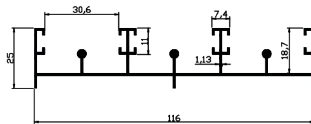
1" 3 Track Bottom
