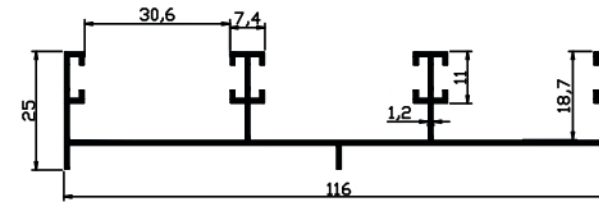
1" 3 Track Top
