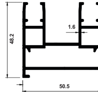
20145 WT KG/12FT=4.370
