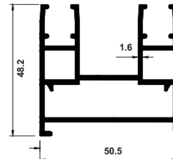
20145 WT KG/12FT=4.370
