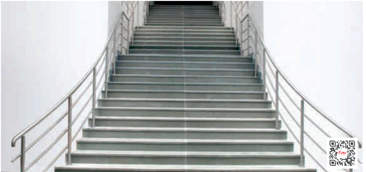
Ø42.4x1.5mm (DT15-1-163) & Ø50x1.5mm (DT12-1-163) Top Mounted Round Baluster System with Horizontal Members
