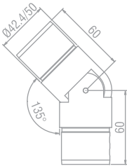
MBHRS - 42.4/50 (S.S. 316) AMBHRS - 42.4/50 (S.S. 304) Smooth Bend for Handrail
