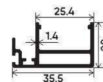
Slim Interlock Shutter 5mm-16mm Glass Shutter Section Number : V-2523 Weight (kg/mt) : 0.468
