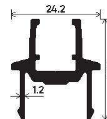
Meeting Section Section Number : V-2935/1744 Weight (kg/12') : 0.410
