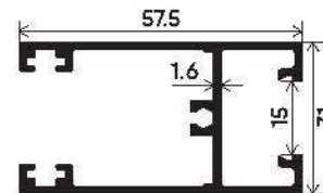
Top Bottom Shutter (Laminated Glass) Section Number : V-3537 Weight (kg/mt) : 0.869
