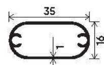
Grill Support Section Number : V-2552 Weight (kg/mt) : 0.276
