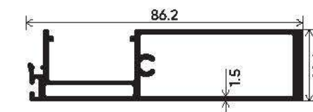
Box Reinforcement Interlock Section Number : V-2930 Weight (kg/mt) : 1.044
