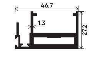
Interlock Heavy Section Number : V-3526 Weight (kg/mt) : 0.989
