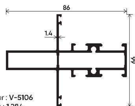
FRAME
