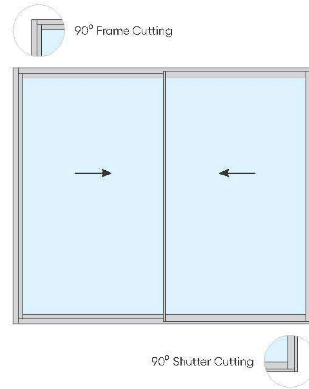
Two Track Shutter Assemble
