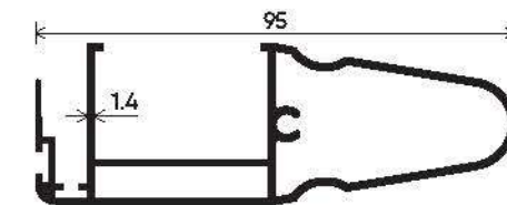
Box Reinforcement DGU Section Number : V-3725 Weight (kg/mt) : 1.085
