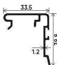
Universal Clip Section Number : V-2921/1746 Weight (kg/mt) : 0.361
