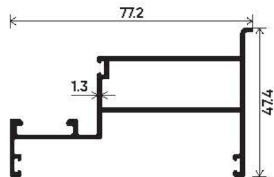
Combination Frame Section Number : V-5112 Weight (kg/mt) : 0.859
