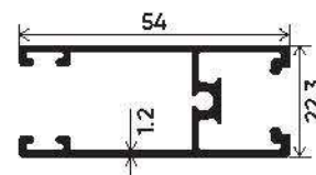
Top Bottom Shutter Section Number : V-2515 Weight (kg/mt) : 0.579
