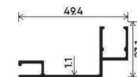
Mosquito Shutter Track Bracket Section Number : V-2510 Weight (kg/mt) : 0.345
