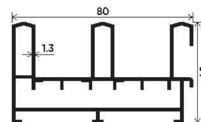
THREE TRACK
