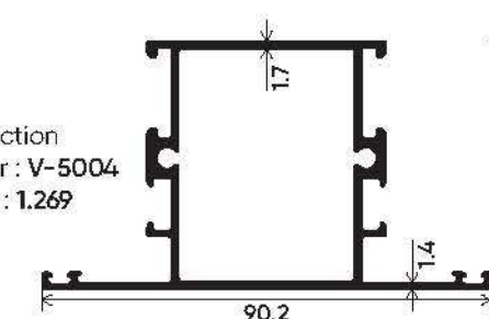
MULLION
