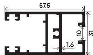
10mm Single Glass Top Bottom Shutter Section Number : V-3539 Weight (kg/mt) : 1.033
