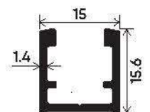
Locking Adapter Section Number : V-3106 Weight (kg/mt) : 0.199
