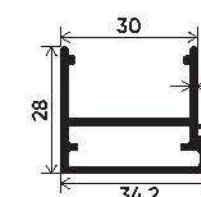
Slim Interlock Shutter 5mm-22mm Glass Shutter Section Number : V-2924 Weight (kg/mt) : 0.561
