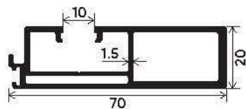
10mm Single Glass Box Reinforcement Interlock Section Number : V-3545 Weight (kg/mt) : 0.988
