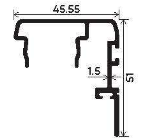
Universal Clip Section Number : V-3771 Weight (kg/mt) : 0.683
