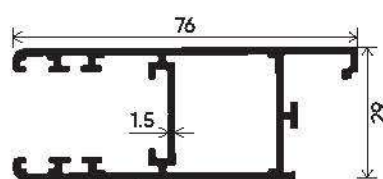
Laminated Shutter With Clip Section Number : V-2917 Weight (kg/mt) : 1.200
