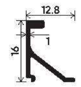
Mosquito Shutter Clip Section Number : V-2514 Weight (kg/mt) : 0.144
