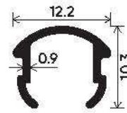
MOSQUITO CLIP
