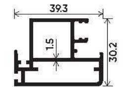
Mosquito Slim Interlock Shutter Section Number : V-3216 Weight (kg/mt) : 0.727
