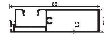
Super Slim Box Reinforcement Interlock Section Number : V-2932 Weight (kg/mt) : 1.050
