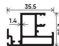
Mosquito Slim Interlock Shutter Section Number : V-2516 Weight (kg/mt) : 0.566
