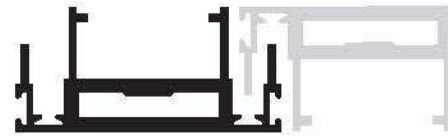
Double Side Interlock Section Number : V-3528 Weight (kg/mt) : 1.150
