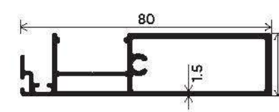
Box Reinforcement Interlock Section Number : V-2527 Weight (kg/mt) : 0.929
