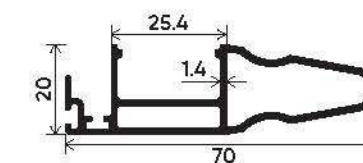
Reinforcement Interlock Shutter 5mm-16mm Glass Shutter Section Number : V-2522 Weight (kg/mt) : 0.803
