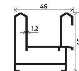
TWO TRACK
