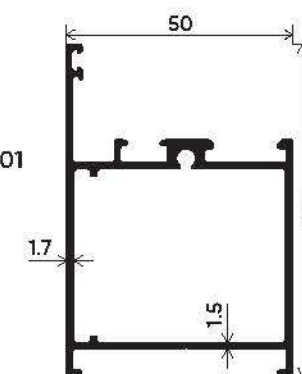
SHUTTER
