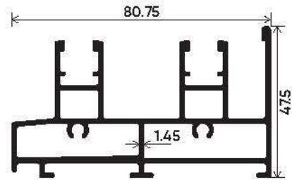
Top & Bottom Track Section Number : V-3103 Weight (kg/mt) : 1.640
