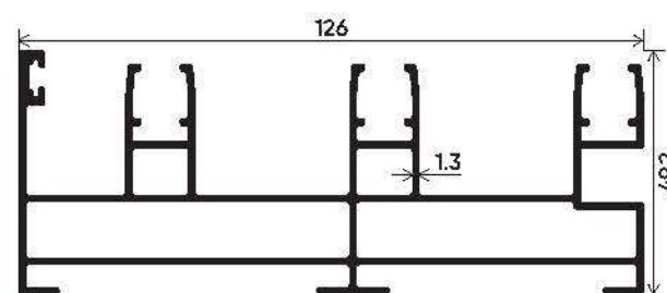
THREE TRACK
