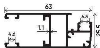
Mosquito Shutter with Screw Pocket Section Number : V-2517 Weight (kg/mt) : 0.900
