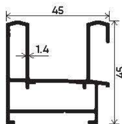
TWO TRACK
