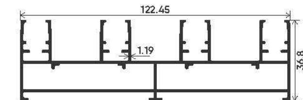
FOUR TRACK
