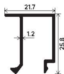
10mm-16mm Glass Clip Section Number : V-5011 Weight (kg/mt) : 0.241
