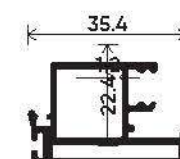
Super Slim Mass Interlock Section Number : V-2933 Weight (kg/mt) : 0.505
