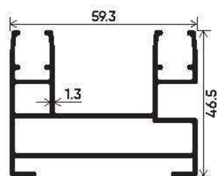
TWO TRACK
