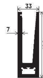
Continuous Railing Bottom Section Number : V-10001 Weight (kg/12') : 15.775
