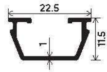
REDUCER CLIP
