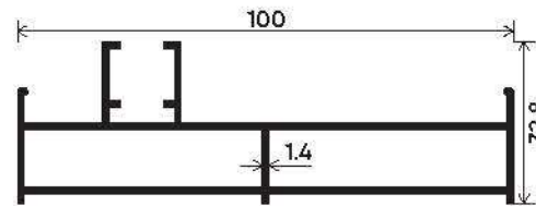
Vertical Track Section Number : V-3501 Weight (kg/mt) : 1.134
