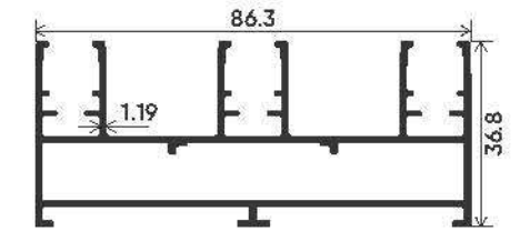
THREE TRACK
