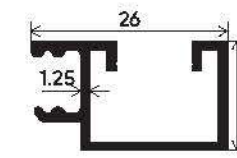
Mosquito Screen Adaptor Section Number : V-3524 Weight (kg/mt) : 0.242
