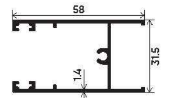
SHUTTER
