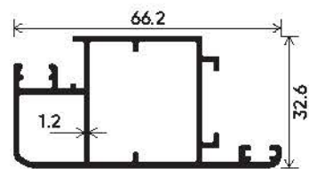
Mesh Shutter Section Number : V-5113 Weight (kg/mt) : 0.779
