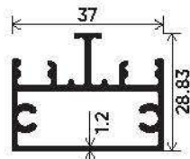
Mosquito Middle Section Section Number : V-2928 Weight (kg/mt) : 0.592
