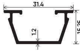
Shutter Glass Reducer Clip Section Number : V-3522 Weight (kg/mt) : 0.211
