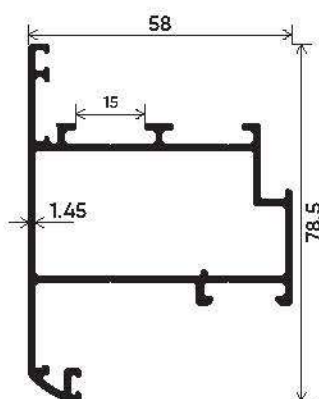
FRAME
