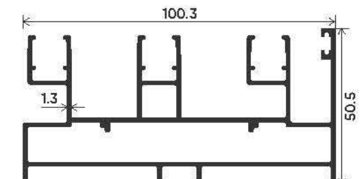
THREE TRACK
