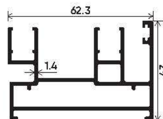
Premium Type Section Number : V-2503 Weight (kg/mt) : 1.168
