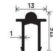
"U" Type Section Number : V-2532 Weight (kg/mt) : 0.166
