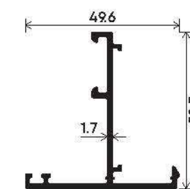
Reverse Adapter Section Number : V-5012 Weight (kg/mt) : 0.497
