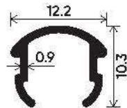
Mosquito Screen Fitting Clip Section Number : V-2524 Weight (kg/mt) : 0.083
