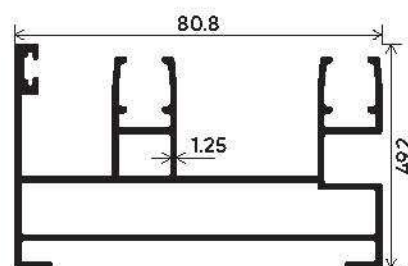
THREE TRACK
