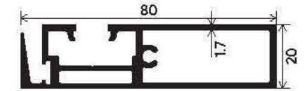
Box Reinforcement Interlock S. G. Section Number : V-3122 Weight (kg/mt) : 1.202
