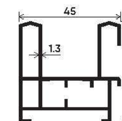
TWO TRACK
