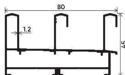
THREE TRACK
