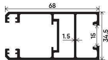
Vertical Shutter (Laminated Glass) Section Number : V-3536 Weight (kg/mt) : 1.066
