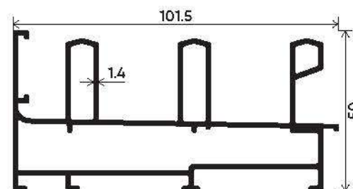
THREE TRACK
