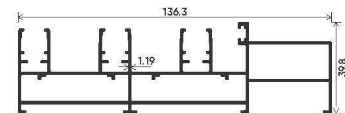
THREE TRACK
