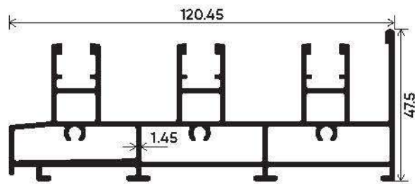
Top & Bottom Track Section Number : V-3104 Weight (kg/mt) : 2.281
