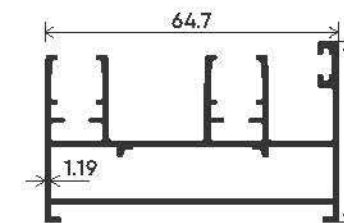
TWO TRACK
