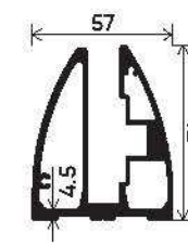
Continuous Railing Bottom Section Number : V-10002 Weight (kg/12') : 9.100
