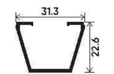
Reducer Clip Section Number : V-3732 Weight (kg/mt) : 0.249
