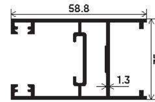
Vertical Shutter Section Number : V-3511 Weight (kg/mt) : 0.891
