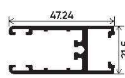
Top & Bottom Shutter Section Number : V-2518 Weight (kg/mt) : 0.620
