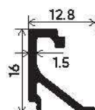
Laminated Shutter Clip Section Number : V-2916 Weight (kg/mt) : 0.134
