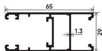
Laminate Shutter Section Number : V-2920 Weight (kg/mt) : 0.798
