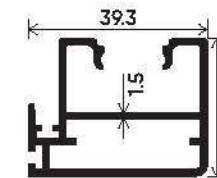
Slim Interlock Shutter SGU Section Number : V-3224 Weight (kg/mt) : 0.692
