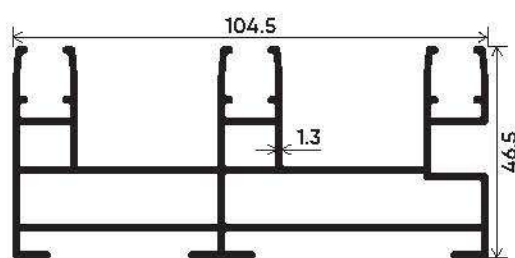
THREE TRACK
