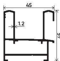
TWO TRACK
