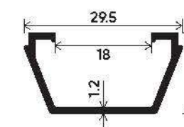
Reducer Clip Laminated Section Number : V-3229 Weight (kg/mt) : 0.195
