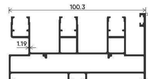
THREE TRACK
