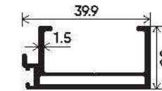
DGU Slim Interlock Section Number : V-3549 Weight (kg/mt) : 0.450
