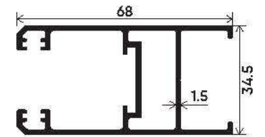
DGU Vertical Shutter Section Number : V-3547 Weight (kg/mt) : 1.000
