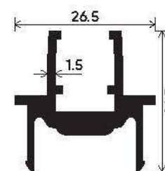
Meeting Section
