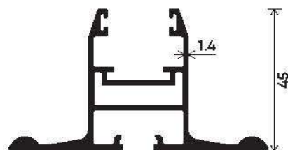
Vertical Shutter SGU Section Number : V-3113 Weight (kg/mt) : 1.100
