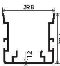
Double Interlocking Clip Section Number : V-2922 Weight (kg/mt) : 0.473
