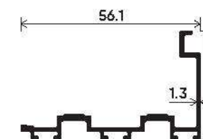
Door Bottom Adapter Section Number : V-5007 Weight (kg/mt) : 0.532
