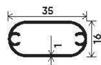
GRILL SUPPORT
