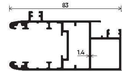
Mosquito Shutter Section Number : V-3713 Weight (kg/mt) : 1.240
