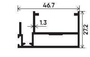
Interlock Section Number : V-3515 Weight (kg/mt) : 0.643
