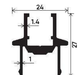
Centre Opening Meeting Section Section Number : V-2525 Weight (kg/mt) : 0.434
