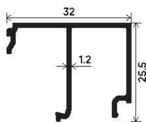
4mm-10mm Glass Clip Section Number : V-5009 Weight (kg/mt) : 0.303
