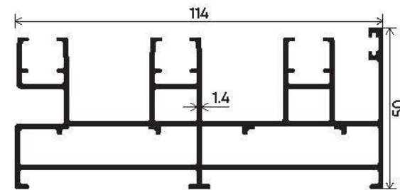
Premium Type Section Number : V-3204 Weight (kg/mt) : 2.099
