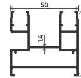
TWO TRACK
