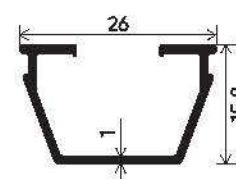
4mm-8mm Glass Section Number : V-2926 Weight (kg/mt) : 0.164
