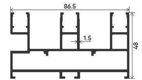
THREE TRACK
