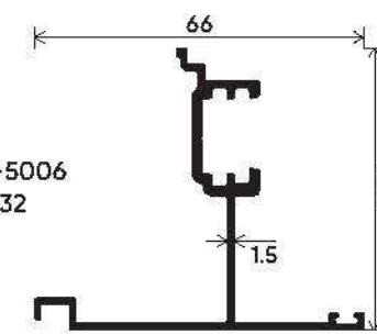
MULLION
