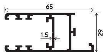
Laminated Shutter With Clip Section Number : V-2915 Weight (kg/mt) : 0.962
