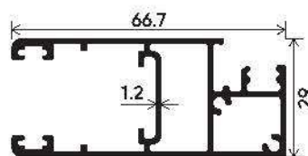
Mosquito Screen Shutter With Screw Section Number : V-2914 Weight (kg/mt) : 0.896
