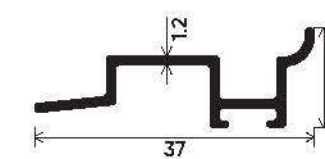
Half Interlock Clip Section Number : V-2520 Weight (kg/mt) : 0.226
