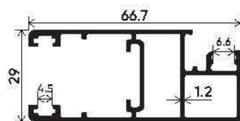
Mosquito Screen Shutter Section Number : V-2913 Weight (kg/mt) : 0.982
