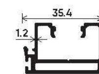
Super Slim Interlock Shutter Section Number : V-2931 Weight (kg/mt) : 0.505
