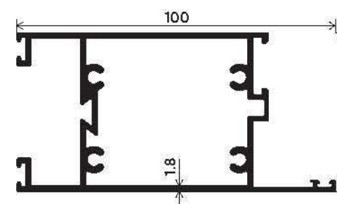
Door Bottom Section Number : V-5005 Weight (kg/mt) : 0.732
