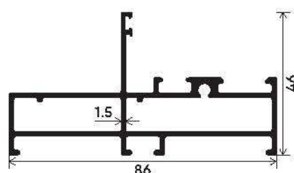
Combination Frame Section Number : V-5104 Weight (kg/mt) : 1.654
