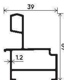
ADDITIONAL TRACK
