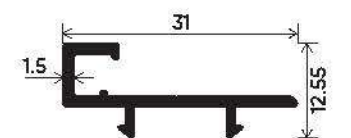
Mosquito Clip Section Number : V-3543 Weight (kg/mt) : 0.206
