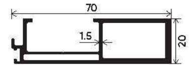
DGU Box Reinforcement Interlock Section Number : V-3550 Weight (kg/mt) : 0.884
