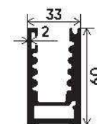
Continuous Railing Bottom Section Number : V-10004 Weight (kg/12') : 6.850
