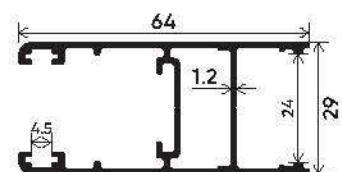
5mm-22mm Glass Shutter Section Number : V-1743/2912 Weight (kg/mt) : 0.849
