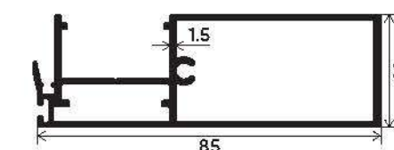
Box Reinforcement Interlock Section Number : V-2927 Weight (kg/mt) : 1.138
