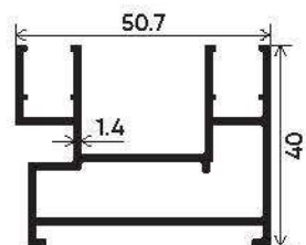
Basic Type Section Number : V-2501 Weight (kg/mt) : 0.883
