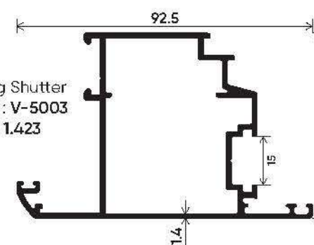
SHUTTER
