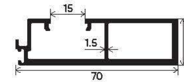
Box Reinforcement Interlock (Laminated Glass) Section Number : V-3542 Weight (kg/mt) : 0.961
