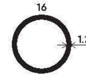
Grill Fitting Tube Cover Section Number : V-1002 Weight (kg/mt) : 0.164
