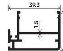
Slim Interlock Shutter 5mm-22mm Glass Shutter Section Number : V-3223 Weight (kg/mt) : 0.596
