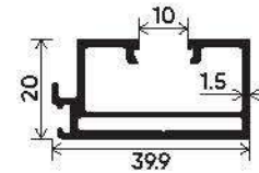
10mm Single Glass Slim Interlock Section Number : V-3544 Weight (kg/mt) : 0.544
