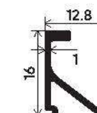
SHUTTER CLIP
