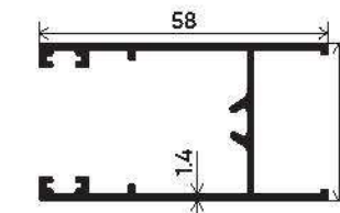
SHUTTER
