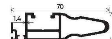
Reinforced Interlock Shutter Section Number : V-2529 Weight (kg/mt) : 0.800
