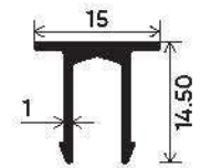
Vertical & Top Track Cover Section Number : V-2533 Weight (kg/mt) : 0.156
