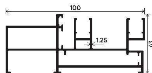
2 in 1 Frame With Grill Section Number : V-2509 Weight (kg/mt) : 1.435
