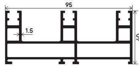
Basic Type Section Number : V-3532 Weight (kg/mt) : 1.870
