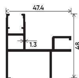
Additional Track Section Number : V-2909 Weight (kg/mt) : 0.700
