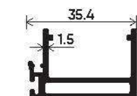
Slim Interlock Shutter Section Number : V-2929 Weight (kg/mt) : 0.503
