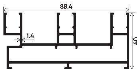
Basic Type Section Number : V-2502 Weight (kg/mt) : 1.417
