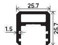
Continuous Railing Top Section Number : V-10053 Weight (kg/12') : 4.600
