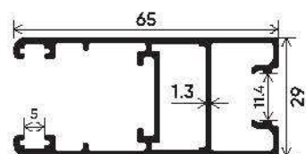
4mm-8mm Glass Shutter Section Number : V-1742/2911 Weight (kg/mt) : 0.942
