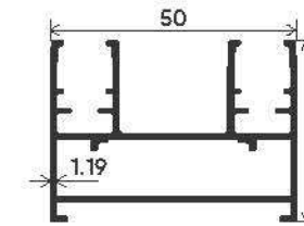
TWO TRACK
