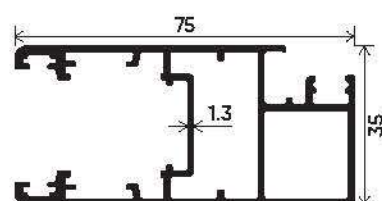
SHUTTER
