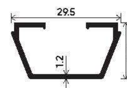
Reducer Clip SGU Section Number : V-3226-1 Weight (kg/mt) : 0.225
