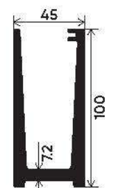
Continuous Railing Bottom Section Number : V-10003 Weight (kg/12') : 14.875
