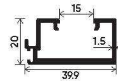
Slim Interlock Shutter (Laminated Glass) Section Number : V-3541 Weight (kg/mt) : 0.525
