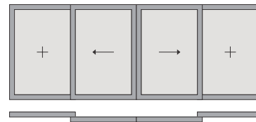
2 TRACK - 4 SHUTTER
