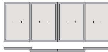
2 TRACK - 4 SHUTTER
