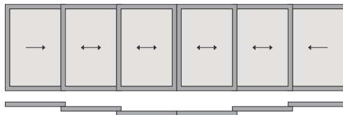
3 TRACK - 6 SHUTTER
