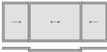
2 TRACK - 3 SHUTTER (X-2X-X)
