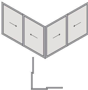
2 TRACK - 4 SHUTTER (CORNER OPENING)
