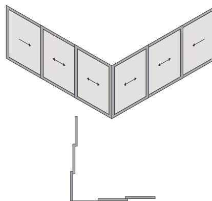
3 TRACK - 6 SHUTTER (CORNER OPENING)
