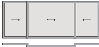
2 TRACK - 3 SHUTTER (X-2X-X)
