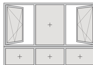
TILT & TURN DOUBLE OPENABLE + CENTER FIX + BOTTOM FIX
