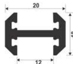
HGP -114 Glass Edge Profile for Partition (Black Matt)
