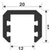
HGP -113 Glass Edge Profile (Black Matt)
