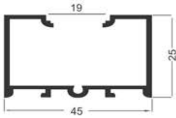
HGP -115 Fix Profile (25x45) Size : 3000mm
