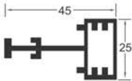
HGP -123 Male Block Profile (25x45) Size : 3000mm
