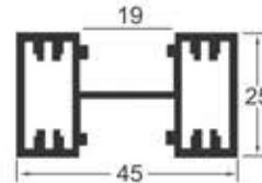
HGP -125 Slim Glaze (25x45) Size : 3000mm
