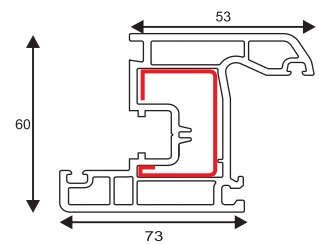
PSPC103 73/60 Casement Window Sash (Inward Open) GI CODE - PSRI 003
