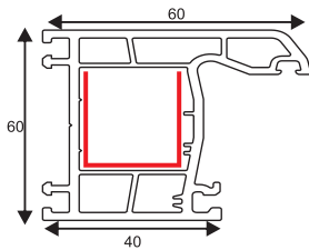
PSPC101 60/60 Casement Outer frame GI CODE - PSRI 008
