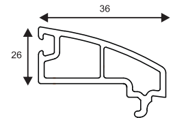
PSPC106 36/26 Casement Single Glazing Bead GI CODE - PSRI 006
