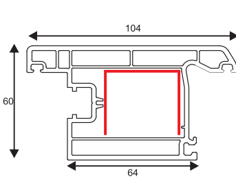
PSPC105 104/60 Casement Door Sash (Outward Open) GI CODE - PSRI 004
