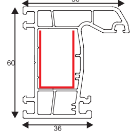
PSPC100 60/56 Casement Outer frame GI CODE - PSRI 015
