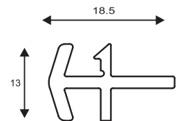
PSPC109 13/19 Coupling (180°) GI CODE - PSRI 008
