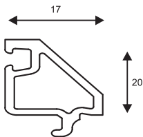
PSPC107 17/20 Casement Double Glazing Bead GI CODE - PSRI 007
