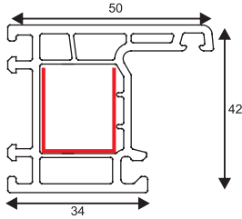
PSPC001 50/42 Casement Outer frame GI CODE - PSRI 005
