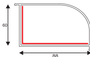
PSPC110 88/60 Bay Pole (90°) GI CODE - PSRI 006
