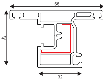
PSPC002 68/42 Casement Outward Sash GI CODE - PSRI 018
