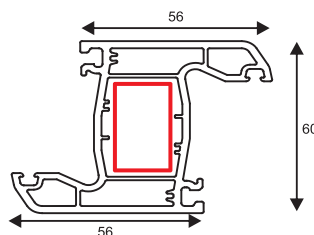
PSPC111 56/60 Casement Z Mullion GI CODE - PSRI 007
