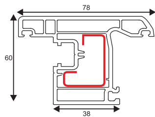
PSPC102 78/60 Casement Window Sash (Outward Open) GI CODE - PSRI 002
