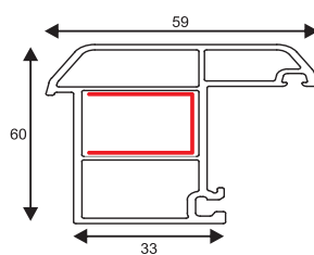
PSPC108 59/60 Casement French Mullion GI CODE - PSRI 005
