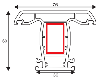
PSPC104 76/60 Transom Mullion GI CODE - PSRI 001
