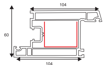
PSPC112 104/60 Casement Door Sash (Inward Open) GI CODE - PSRI 004
