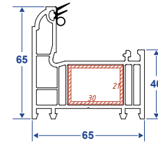
NAME:65 frame CODE:FTM65K WEIGHT(KG/M):1.25 PCS/BAG:6 THICKNESS:2.5
