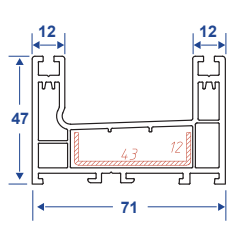
NAME:71 sliding frame CODE:FT71TLKB WEIGHT(KG/M):1.10 PCS/BAG:6 THICKNESS:2.3
