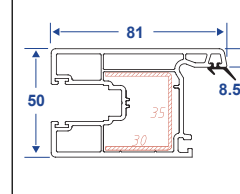
NAME:50-81 sash CODE:FT50S81 WEIGHT(KG/M):1.362 PCS/BAG:6 THICKNESS:2.4
