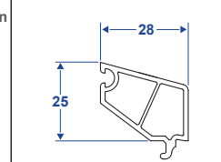
NAME:glazing bead 28 CODE:FTM70SY-28 WEIGHT(KG/M):0.283 PCS/BAG:20 THICKNESS:1.2
