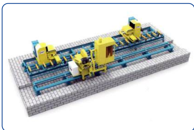
Hydraulic , flat rail, handover type three-head puller
