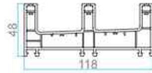
AP 302 A SLIDING INTERMEDIATE FRAME 3-TRACK
