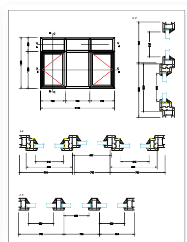
CAD cross-section
