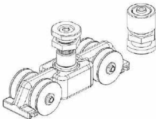
Bogie Set
