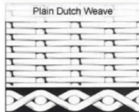
Plain Dutch Weave
