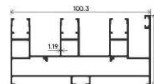
THREE TRACK
