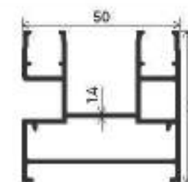
TWO TRACK
