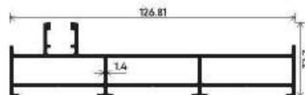
Vertical Track Section Number : V-3105 Weight (kg/mt) : 0.941
