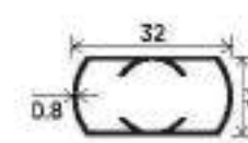
Grill Support Pipe with Safety rod Section Number : V-2553 Weight (kg/mt) : 0.250
