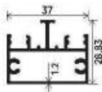
MIDDLE SHUTTER
