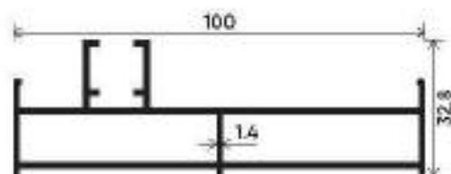
Vertical Track Section Number : V-3501 Weight (kg/mt) : 1.134
