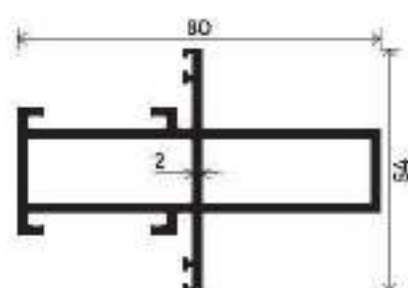
KPA MULLION
