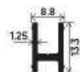
TRACK RAIL CAP
