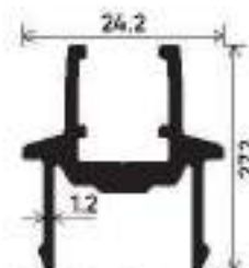
Meeting Section Section Number : V-2935/1744 Weight (kg/12') : 0.410
