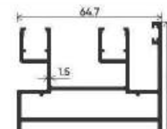
TWO TRACK
