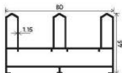
Regular Type Section Number : V-2717 Weight (kg/12') : 4.280
