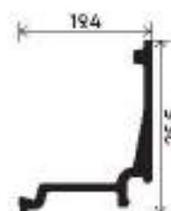
40mm Glass Round Clip Section Number : V-5013 Weight (kg/mt) : 0.173
