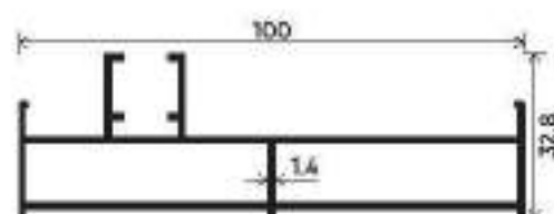
TWO TRACK SIDE
