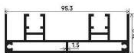
TWO TRACK
