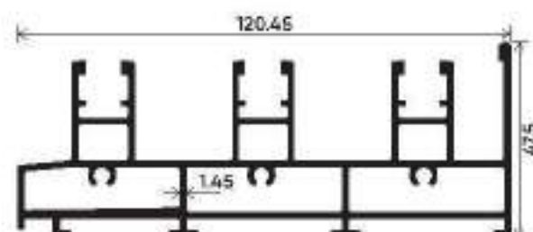
Top & Bottom Track Section Number : V-3104 Weight (kg/mt) : 2.281
