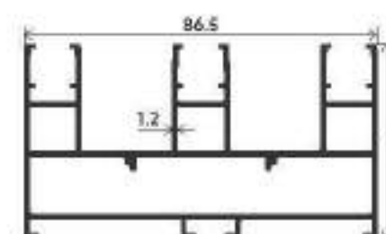
THREE TRACK
