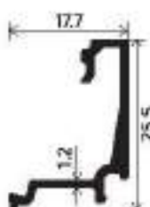
35mm Glass Clip Section Number : V-5015 Weight (kg/mt) : 0.198
