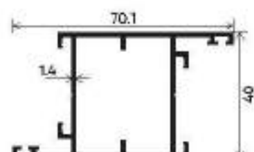
SHUTTER
