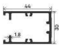
REINFORCEMENT
