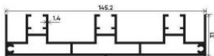
Top & Bottom Track Section Number : V-3505 Weight (kg/mt) : 2.073
