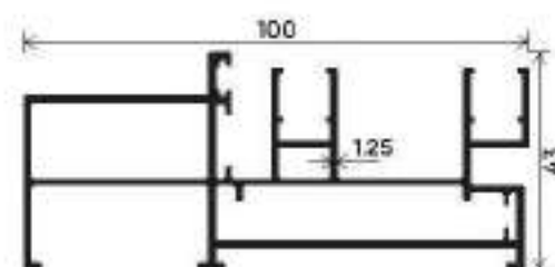
TWO TRACK
