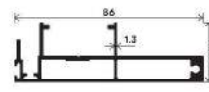
40mm Reinforcement Interlock Shutter Section Number : V-3517 Weight (kg/mt) : 0.977
