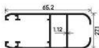
Handle Domal Section Number : V-2726/1753 V-2726/1754 Weight (kg/12') : 2.450 2.800
