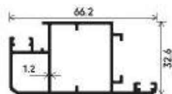
SHUTTER
