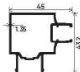
Corner Windows Shutter Section Number : V-2918 Weight (kg/mt) : 0.655
