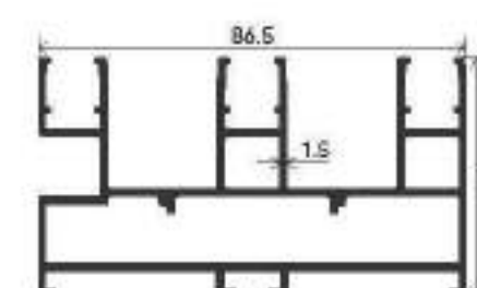
THREE TRACK
