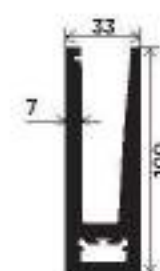
Continuous Railing Bottom Section Number : V-10001 Weight (kg/12') : 15.775
