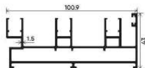
THREE TRACK
