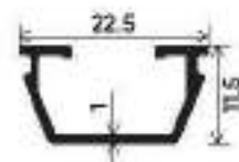
REDUCER CLIP
