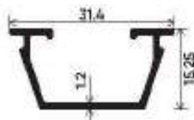
REDUCER CLIP
