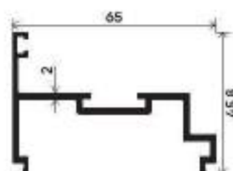
S & F ADAPTOR
