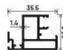
SHUTTER
