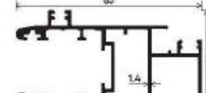
SHUTTER
