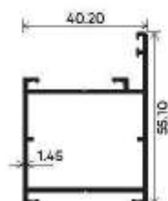
BOX FRAME
