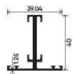
MULLION
