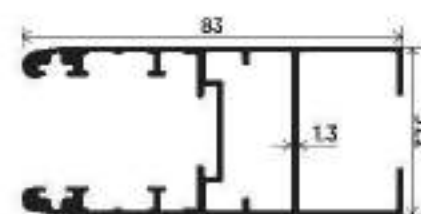
SHUTTER
