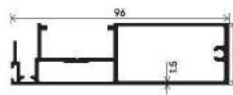
Box Reinforcement Interlock Section Number : V-3516-1 Weight (kg/mt) : 1.179
