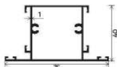
SHUTTER
