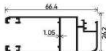
Mosquito Shutter Section Number : V-2727/1756 Weight (kg/12') : 2.500
