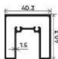
Continuous Railing Top Section Number : V-10052 Weight (kg/12') : 3.400
