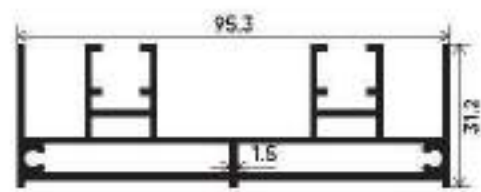
Top & Bottom Track Section Number : V-3502 Weight (kg/mt) : 1.544
