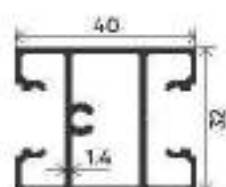
MIDDLE SECTION
