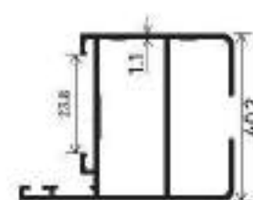
MIDDLE SECTION
