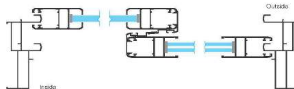
Top View
