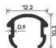
MOSQUITO CLIP
