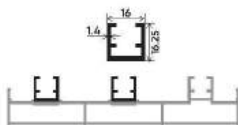
Vertical Track Section Number : V-3504 Weight (kg/mt) : 0.245
