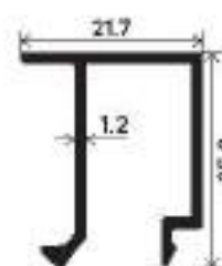
10mm-16mm Glass Clip Section Number : V-5011 Weight (kg/mt) : 0.241
