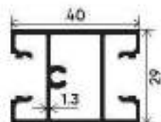
Middle Shutter Section Number : V-2925 Weight (kg/mt) : 0.683
