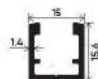
Locking Adapter Section Number : V-3106 Weight (kg/mt) : 0.199
