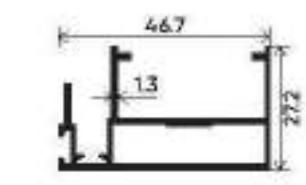
Interlock Section Number : V-3515 Weight (kg/mt) : 0.643
