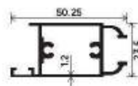
Mosquito Shutter Section Number : V-4010/1355 Weight (kg/mt) : 0.669
