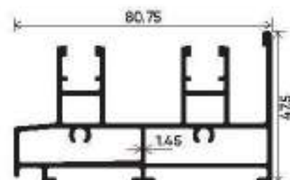
Top & Bottom Track Section Number : V-3103 Weight (kg/mt) : 1.640
