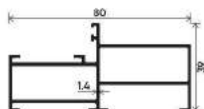
FRAME
