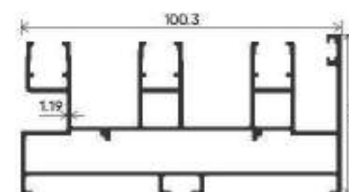
THREE TRACK
