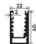
Continuous Railing Bottom Section Number : V-10004 Weight (kg/12') : 6.850
