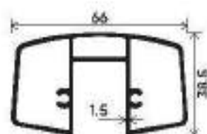
Continuous Railing Top Section Number : V-10054 Weight (kg/12') : 4.080
