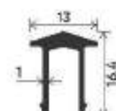
TRACK RAIL CLIP
