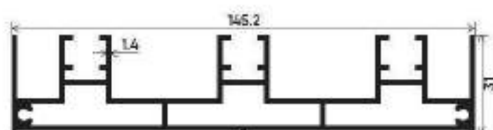
THREE TRACK
