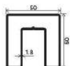
Continuous Railing Top Section Number : V-10053 Weight (kg/12') : 4.600
