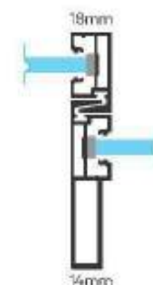
Slim Interlock SGU
