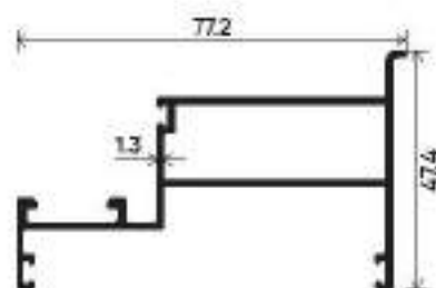
Combination Frame Section Number : V-5112 Weight (kg/mt) : 0.859
