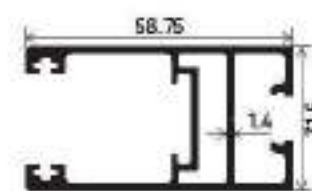
Vertical S. G. Shutter Section Number : V-3111 Weight (kg/mt) : 0.942
