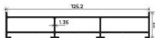
Vertical Track Plain Section Number : V-3107 Weight (kg/mt) : 1.300
