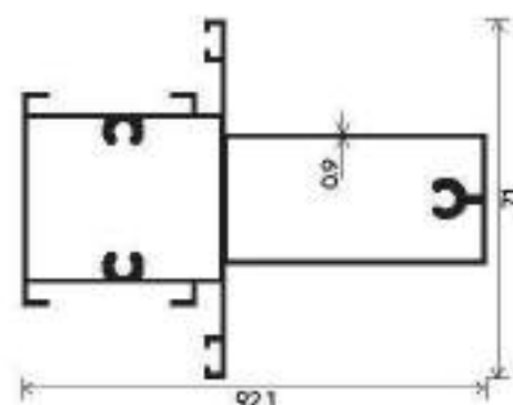
KPA MULLION
