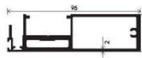
Box Reinforcement Interlock Heavy Section Number : V-3527 Weight (kg/mt) : 1.761
