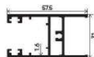
DGU Top Bottom Shutter Section Number : V-3548 Weight (kg/mt) : 0.928
