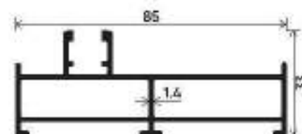
Vertical Track Section Number : V-3102 Weight (kg/mt) : 1.04
