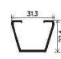
REDUCER CLIP
