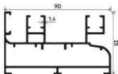
TWO TRACK
