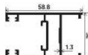
Vertical Shutter Section Number : V-3511 Weight (kg/mt) : 0.891
