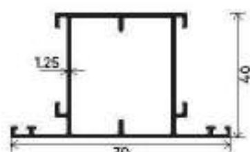
SHUTTER
