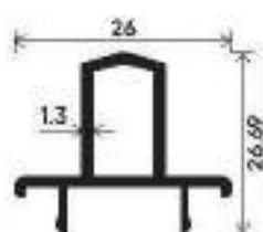
Meeting Section Section Number : V-2743/L-2 Weight (kg/12') : 0.900
