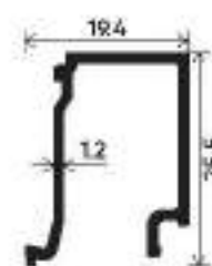
16mm-24mm Glass Clip Section Number : V-5008 Weight (kg/mt) : 0.226
