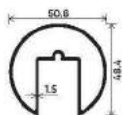
Continuous Railing Top Section Number : V-10051 Weight (kg/12') : 3.200
