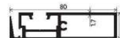
Box Reinforcement Interlock S. G. Section Number : V-3122 Weight (kg/mt) : 1.202
