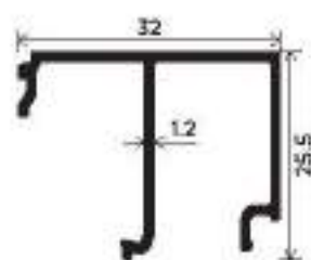
4mm-10mm Glass Clip Section Number : V-5009 Weight (kg/mt) : 0.303
