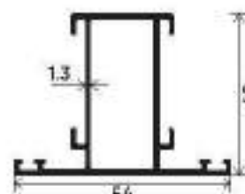
ECO MULLION
