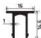
Track Cover Cap Section Number : V-2533 Weight (kg/mt) : 0.140
