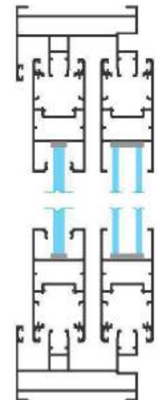
Side View
