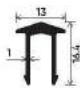
"V" Type Section Number : V-2531 Weight (kg/mt) : 0.156
