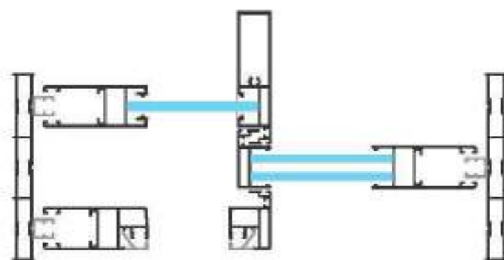
Section Detail
