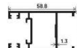
Vertical Shutter Premium Section Number : V-3530 Weight (kg/mt) : 0.891
