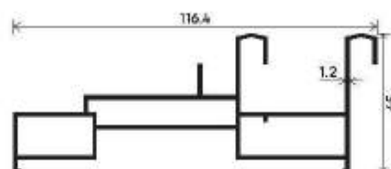
2 Track Grill With Mosquito Section Number : V-2742/1809 Weight (kg/12') : 4.450
