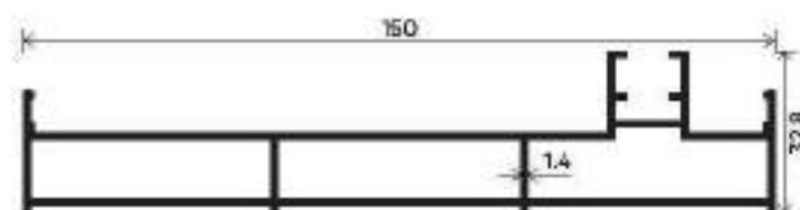
Plain Vertical Track Section Number : V-3510 Weight (kg/mt) : 1.566
