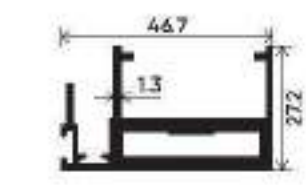
Interlock Heavy Section Number : V-3526 Weight (kg/mt) : 0.989
