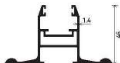
Vertical Shutter DGU Section Number : V-3114 Weight (kg/mt) : 1.168
