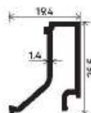
30mm Glass Clip Section Number : V-5014 Weight (kg/mt) : 0.247
