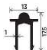
"U" Type Section Number : V-2532 Weight (kg/mt) : 0.166
