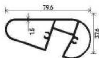
Continuous Railing Top Section Number : V-10055 Weight (kg/12') : 4.100
