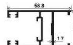
Vertical Shutter Heavy Section Number : V-3514 Weight (kg/mt) : 0.930
