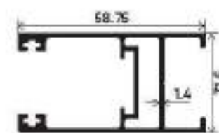
Vertical DGU Shutter Section Number : V-3115 Weight (kg/mt) : 0.942
