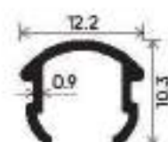
Mosquito Screen Fitting Clip Section Number : V-2524 Weight (kg/12') : 2.900
